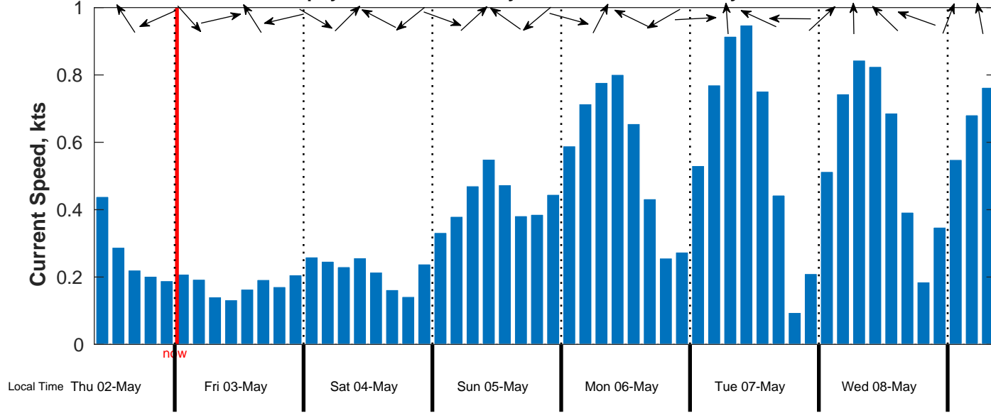
Current Forecast for Shell Zephyrus GT from 03-May-2024 00:00:00 to 10-May-2024 00:00:00
